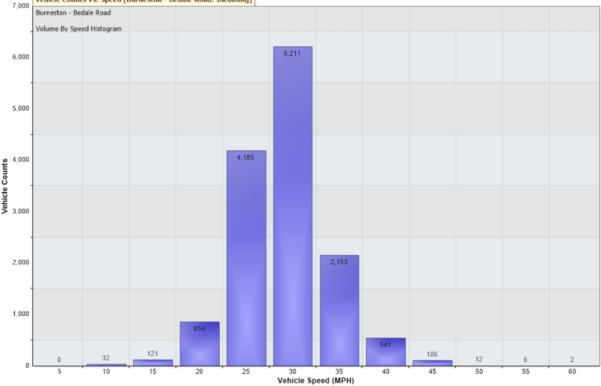
Vehicle Counts Vs. Speed [Burneston - Bedale Road: Incoming]
